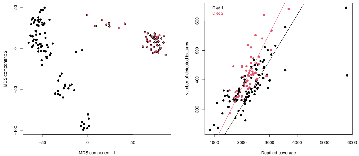
Figure 5: Left) CMDS of features (plotOrd). Right) Rarefaction effect (plotRare).
