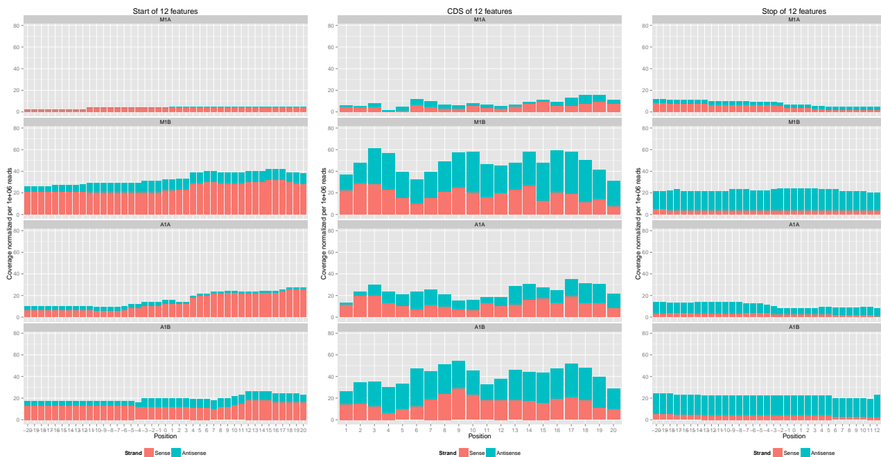
Figure 4: Feature coverage plot with single nucleotide resolution around start and stop codons and binned coverage between them
