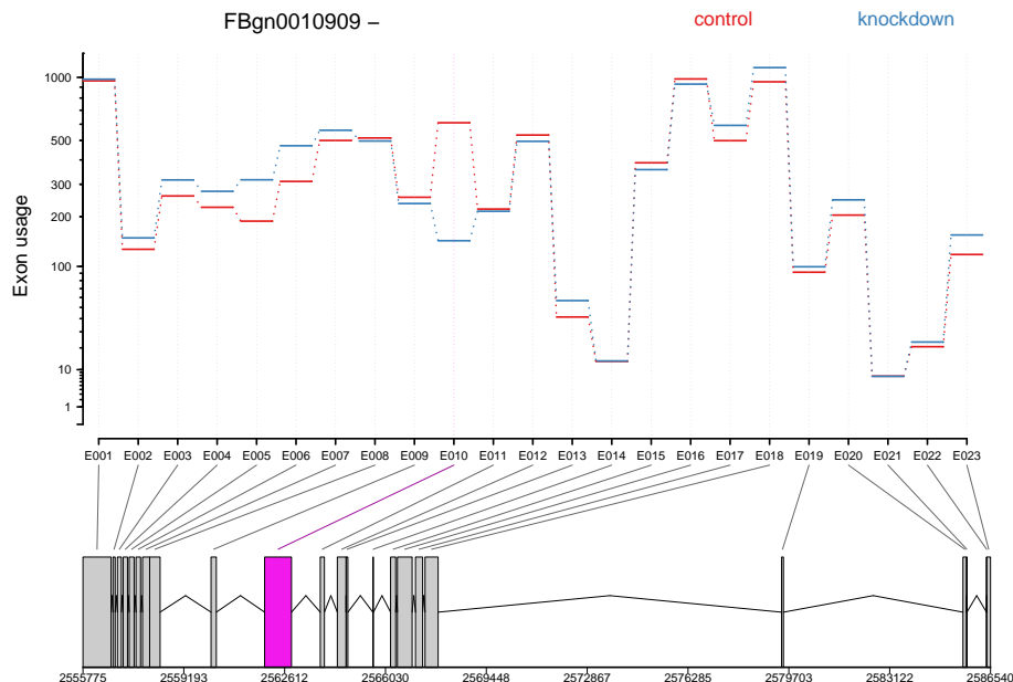
Figure 6: Fitted splicing
