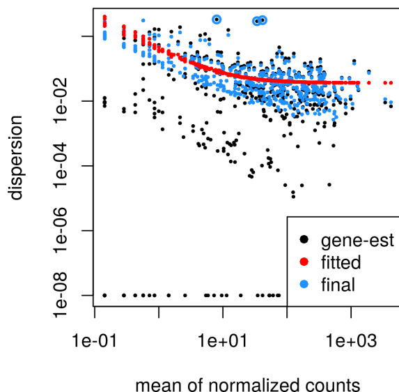
Figure 1: Fit Diagnostics
