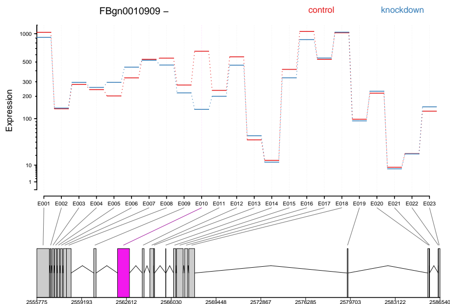
Figure 3: Fitted expression
