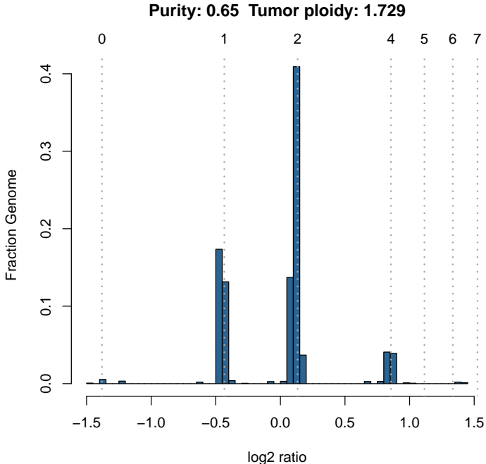
Figure 3: Log-ratio histogram.
