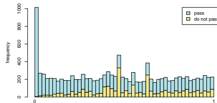
Figure 5: Histogram of p -values for all tests
