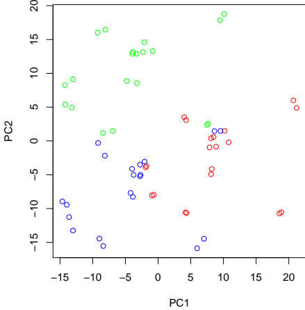
(c) hclust - colored by Tissue
