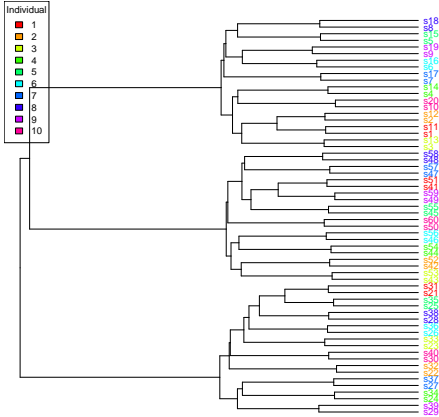
(f) variancePartition - within Tissue
