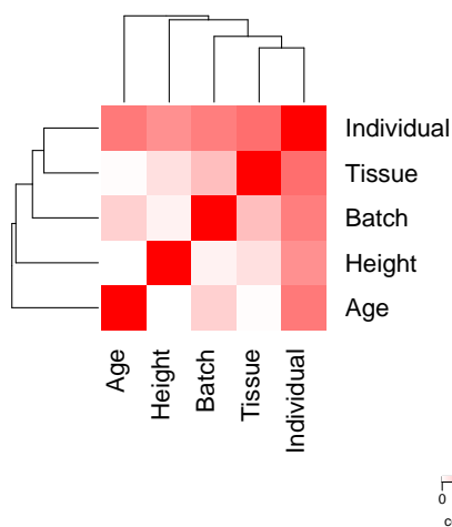
Figure 3: Assess correlation between all pairs of variables
